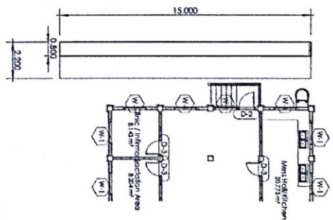
3 A101 Ground Floor Plan 1 : 200
