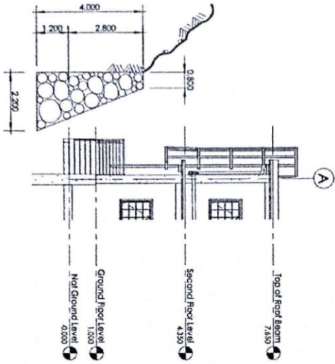
4 A101 Front View 1 : 125
