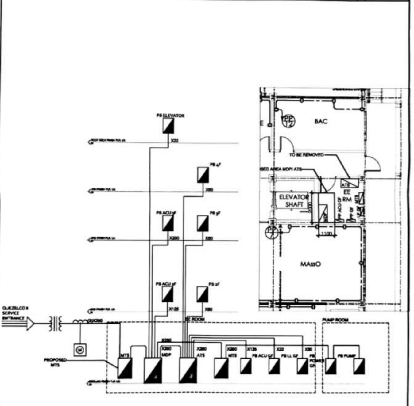
1 SINGLE LINE RISER DIAGRAM E - NOT TO SCALE
